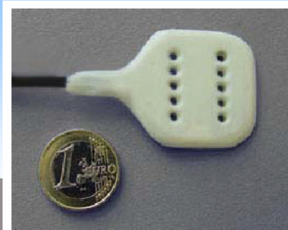
Layout and size of the Fiberoptical Sensor
